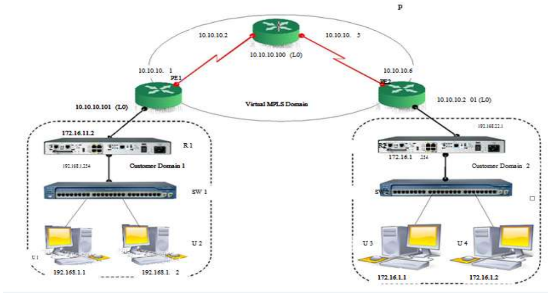
Configuration methods of Embedded IP/MPLS based model Figure 2 represents the Snapshot of IP/MPLS embedded network model.
